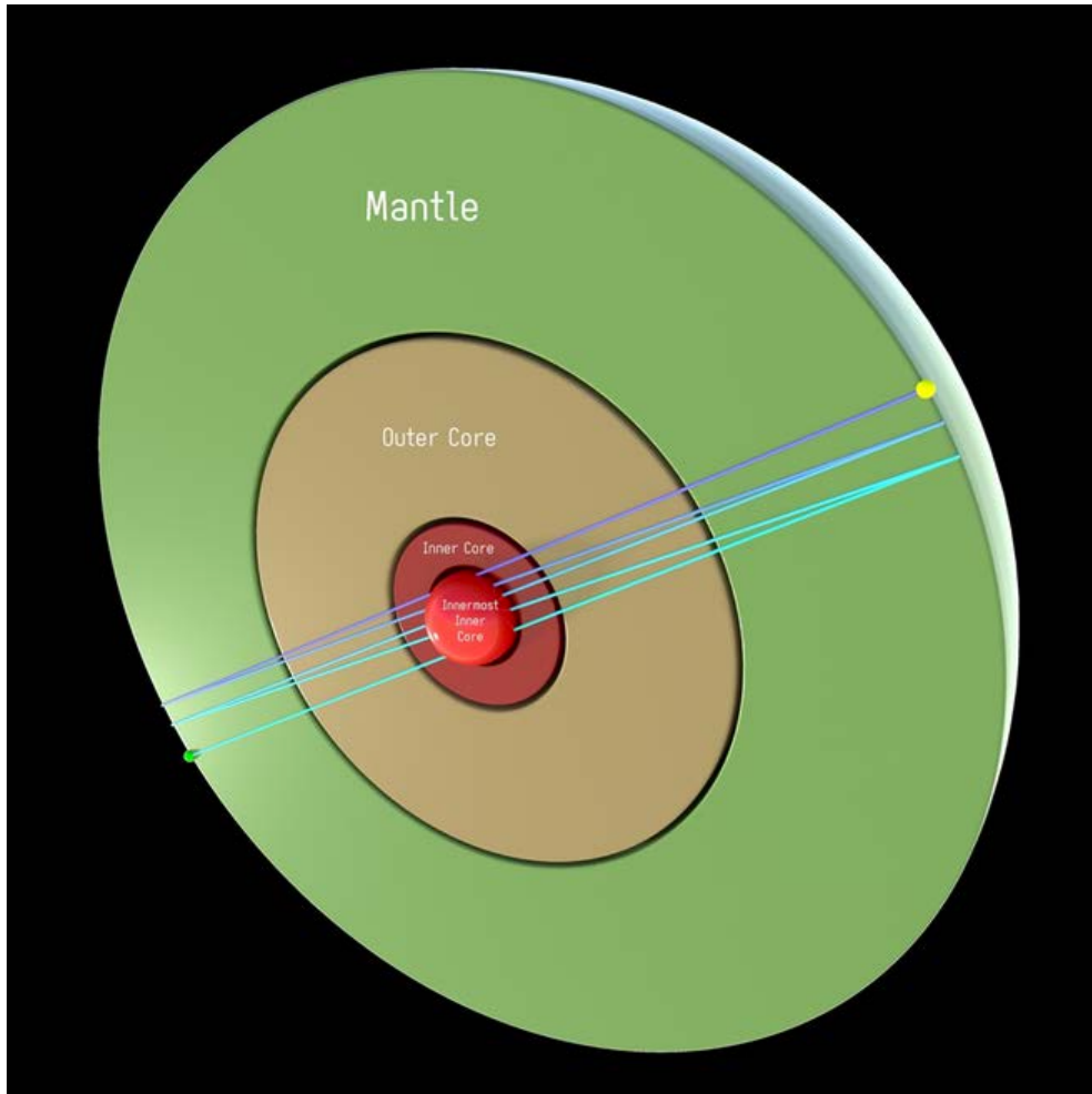
A simple illustration of the ricochet waves through the Earth's innermost inner core (Phạm and Tkalčić, Nature Communications, 2023). This illustration appeared on the front page of New York Times, and other outlets worldwide.
