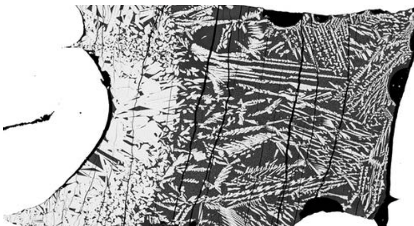
A back-scattered electron image of a high pressure experimental run showing primary and quench monazite crystals in a quenched carbonate-phosphate melt. Courtesy Srijita Ray, PhD student in Experimental Petrology.
