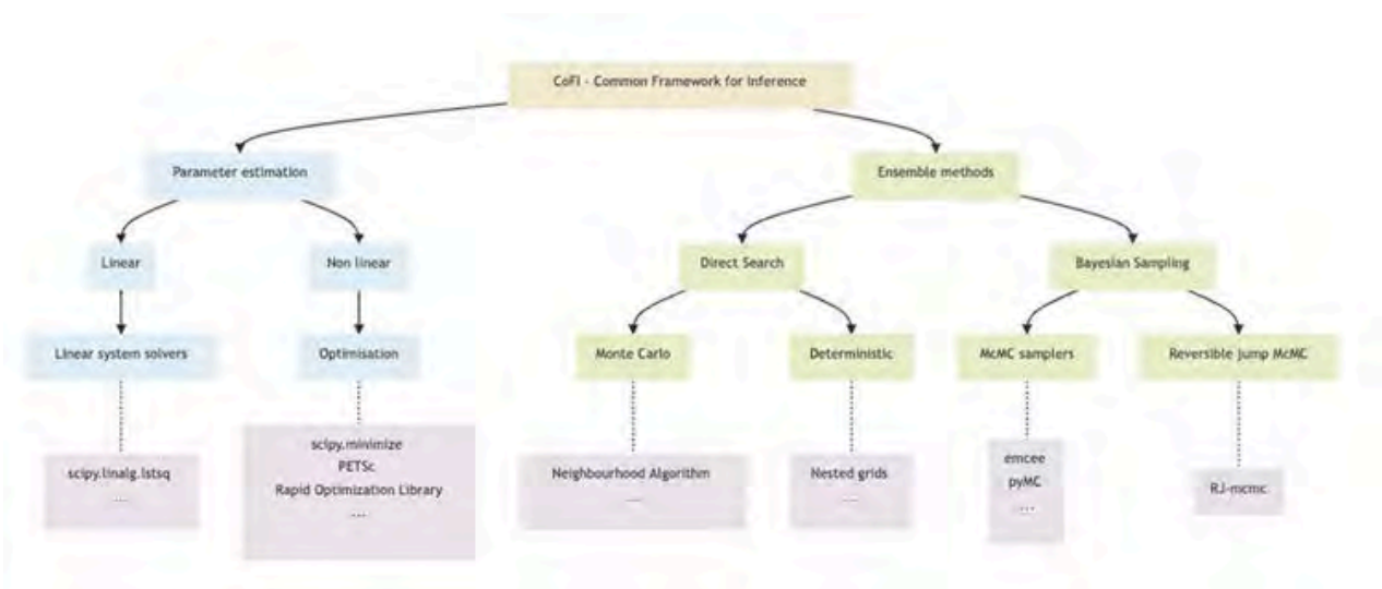
Overview of the inference tools available through CoFI.
